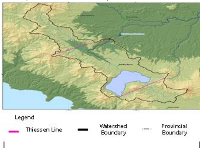
Figure 3. Thiessen Polygon Map of the Tiga Dihaji Dam Watershed
